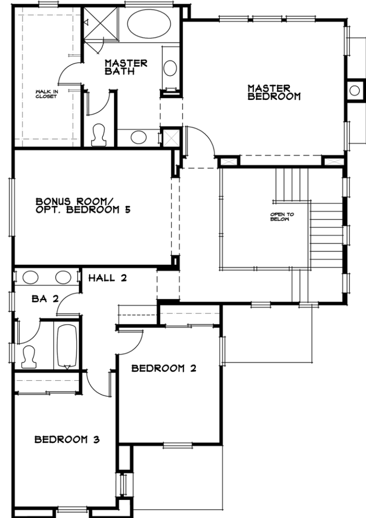
SECOND FLOOR PLAN 2
