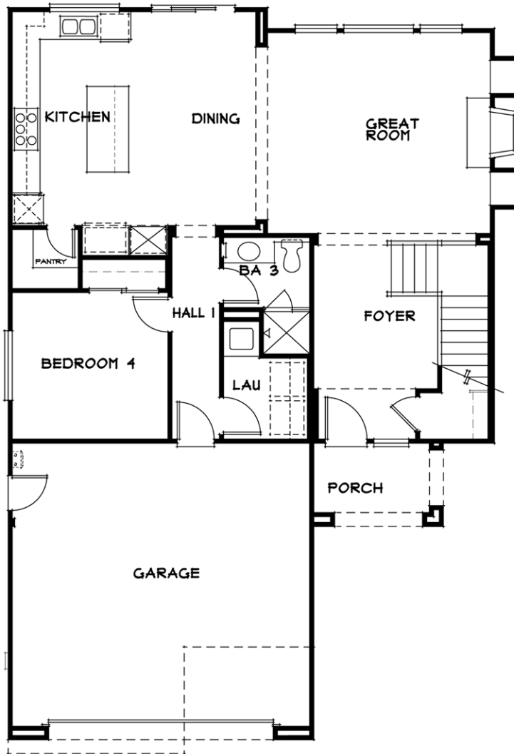
FIRST FLOOR PLAN 2
