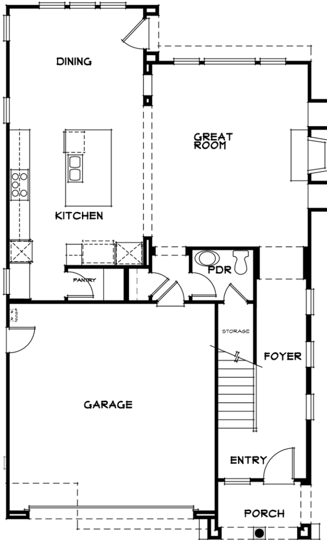
FIRST FLOOR PLAN 1
